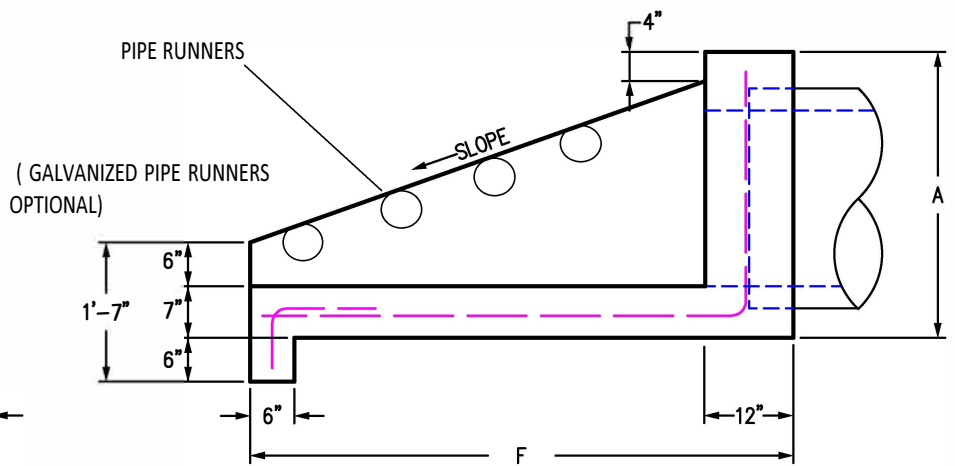
ELEVATION VIEW
