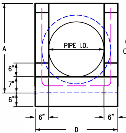
SECTION VIEW
