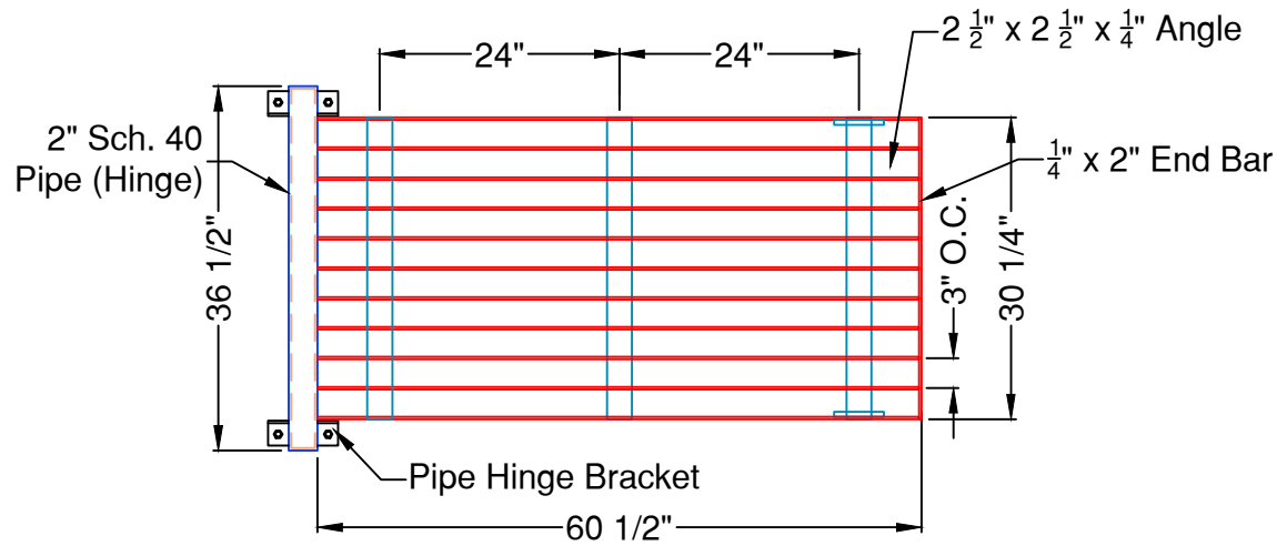
Side Assembly Plan View
